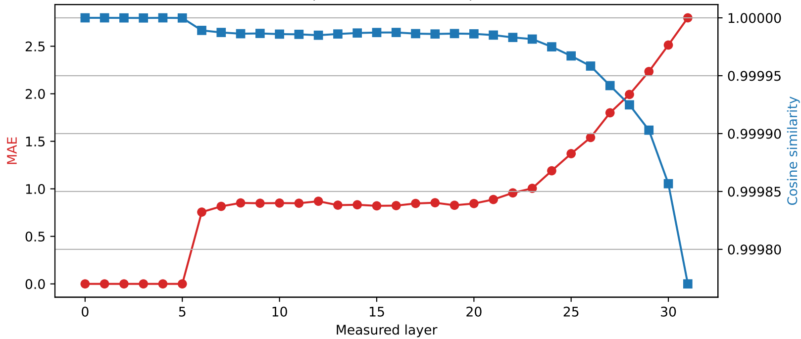
SmolLM2-360M | Quantized layer 5 | float16 → int2
