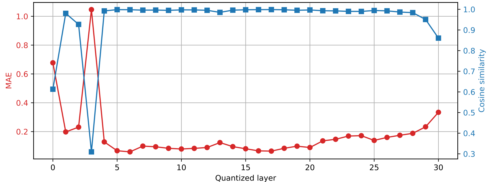
SmolLM2-360M | Prompt 4 Final RMSNorm output damage | float16 \rightarrow int2
