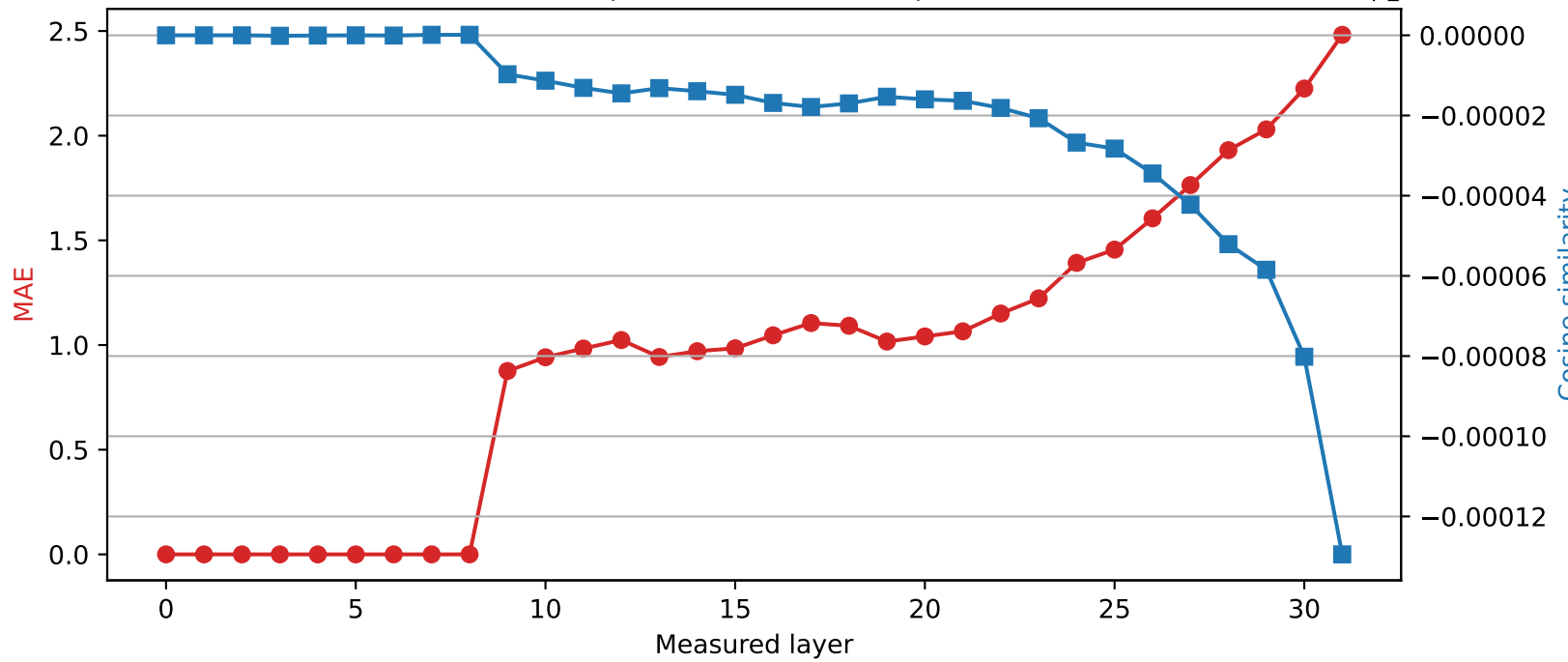
SmolLM2-360M | Quantized layer 8 | float16 \rightarrow int2
