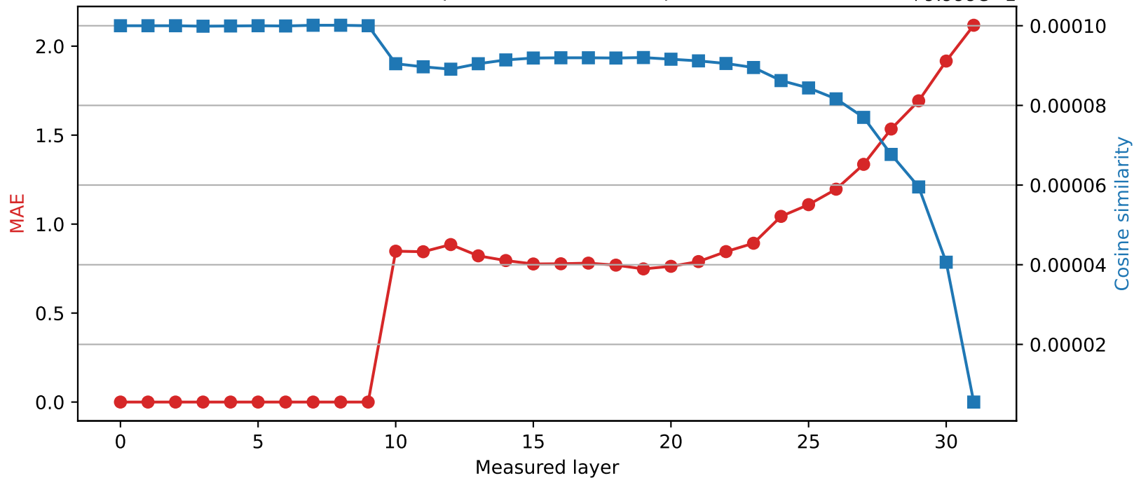
SmolLM2-360M | Quantized layer 9 | float16 → int2
