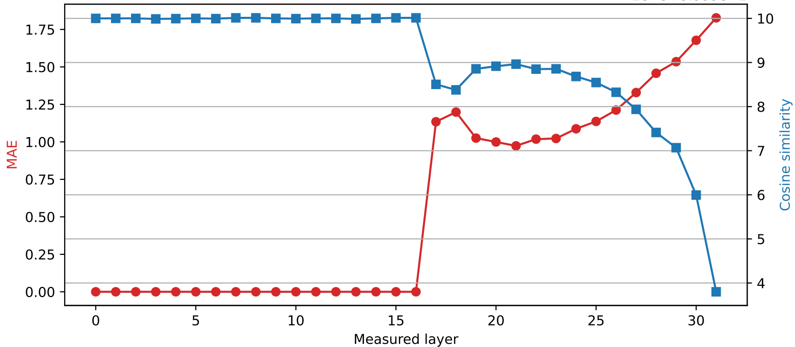
SmolLM2-360M | Quantized layer 16 | float16 \rightarrow int2 1e-5+9.999e-1
