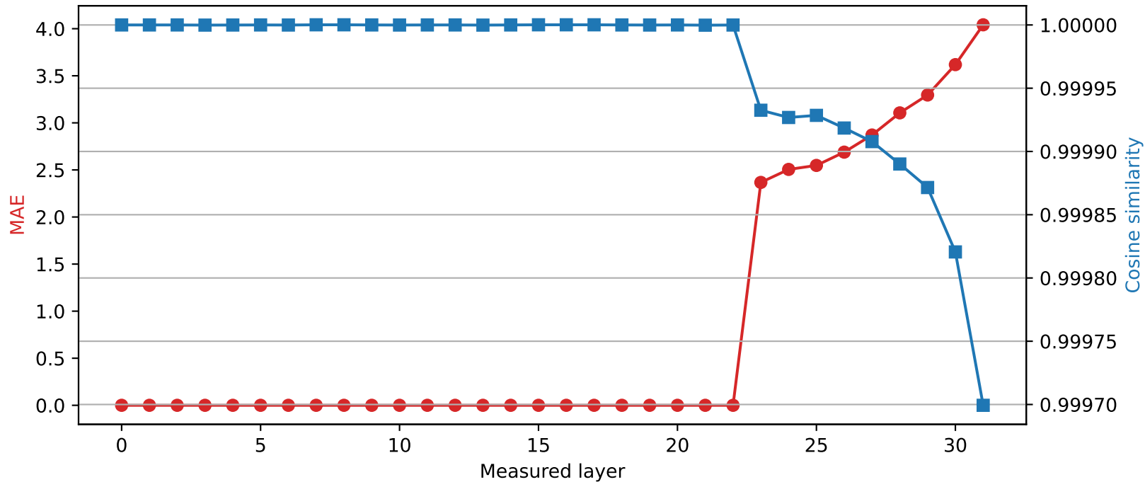
SmolLM2-360M | Quantized layer 22 | float16 → int2
