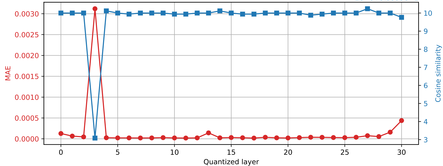
SmolLM2-360M | Prompt 0 Final RMSNorm output damage | float32 → int16
