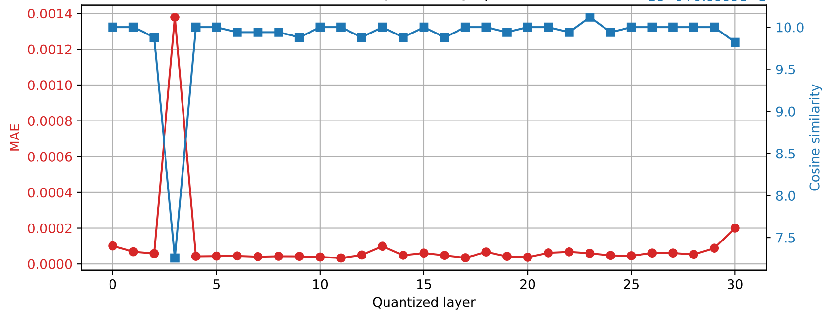
SmolLM2-360M | Prompt 1 Final RMSNorm output damage | float32 \rightarrow int16
