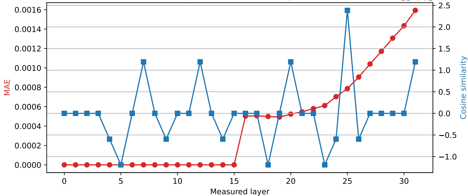
SmolLM2-360M | Quantized layer 15 | float32 \rightarrow int16
