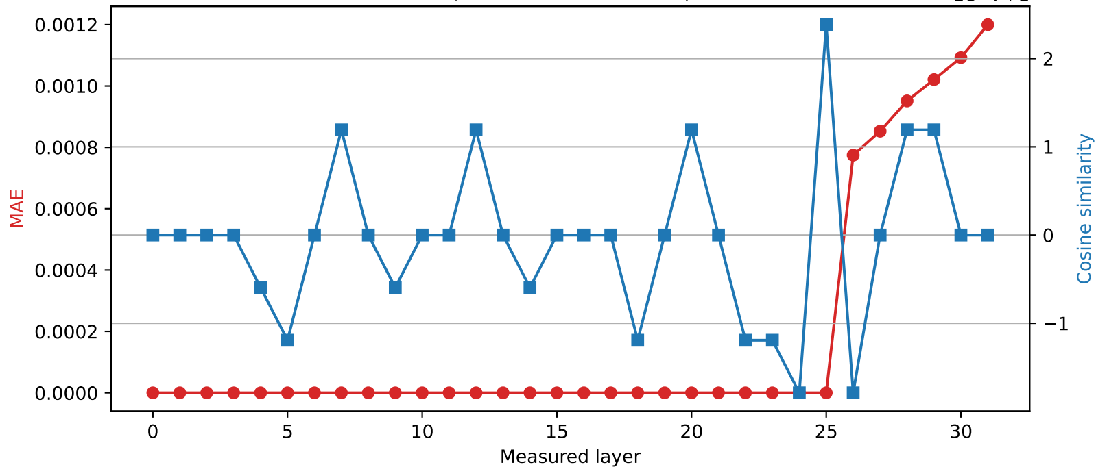
SmolLM2-360M | Quantized layer 25 | float32 \rightarrow int16
