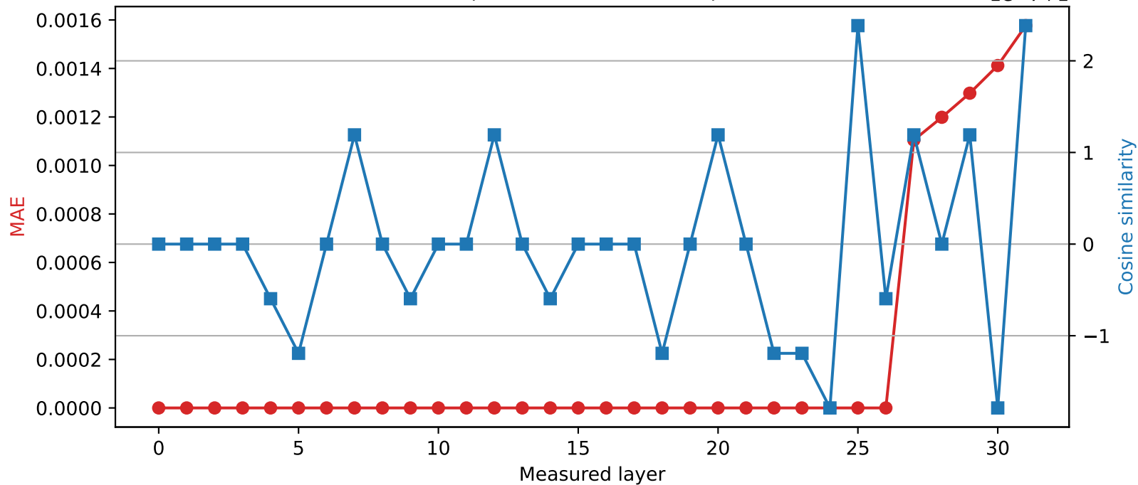
SmolLM2-360M | Quantized layer 26 | float32 \rightarrow int16
