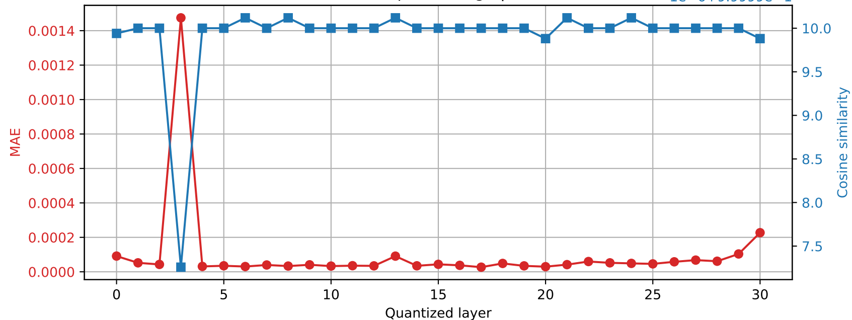
SmolLM2-360M | Prompt 2 Final RMSNorm output damage | float32 → int16
