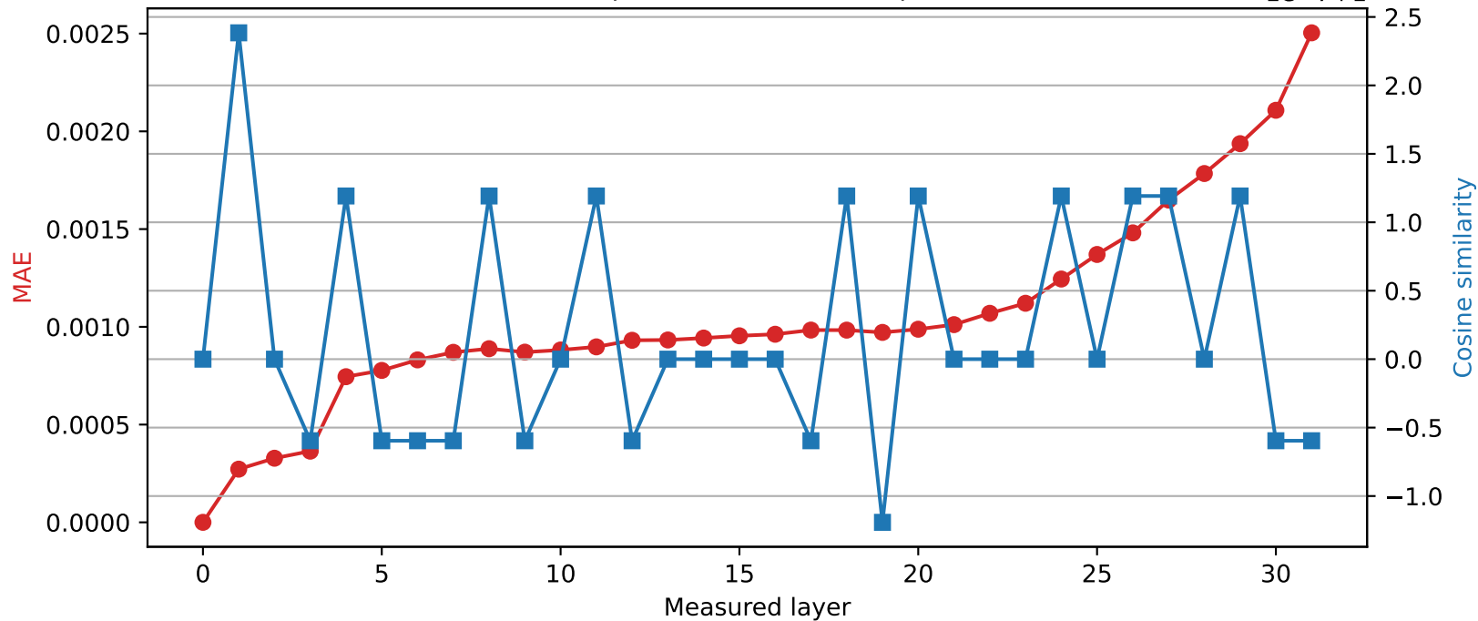
SmolLM2-360M | Quantized layer 0 | float32 \rightarrow int16
