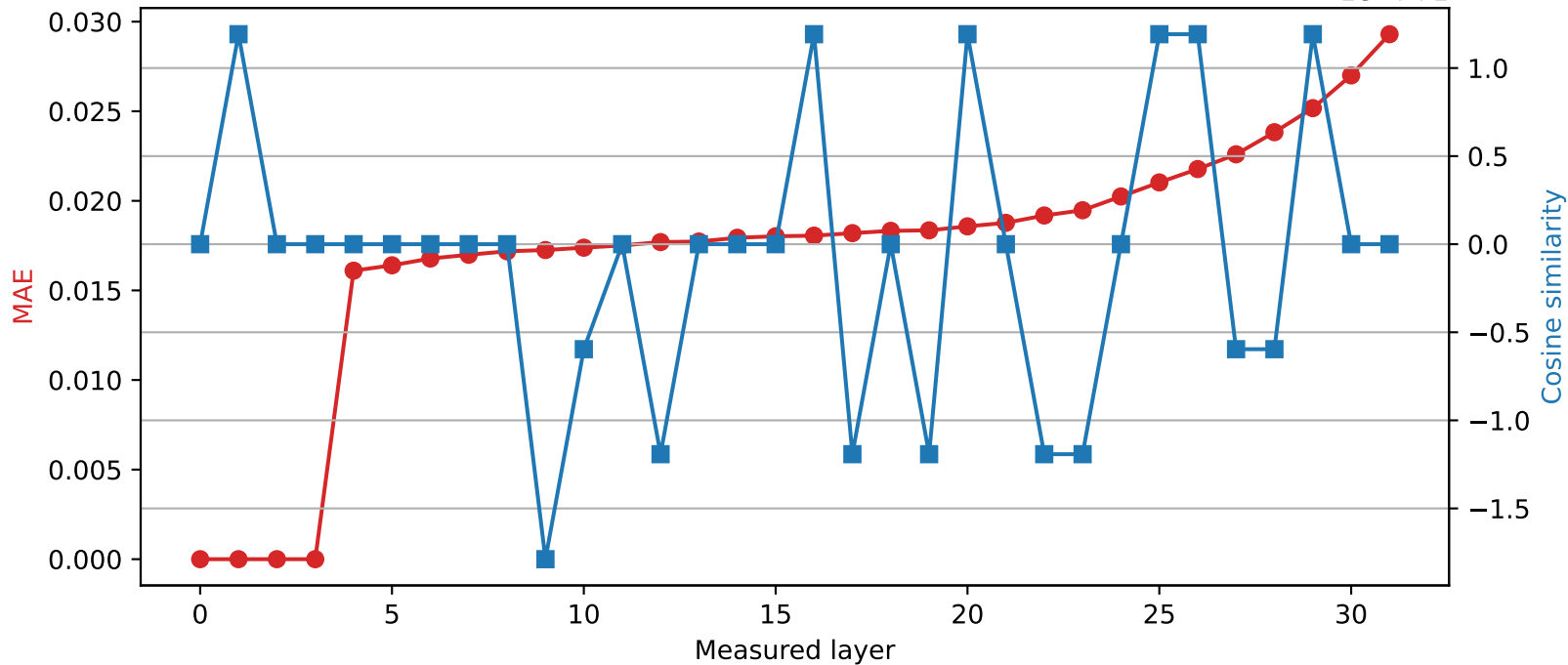
SmolLM2-360M | Quantized layer 3 | float32 \rightarrow int16
