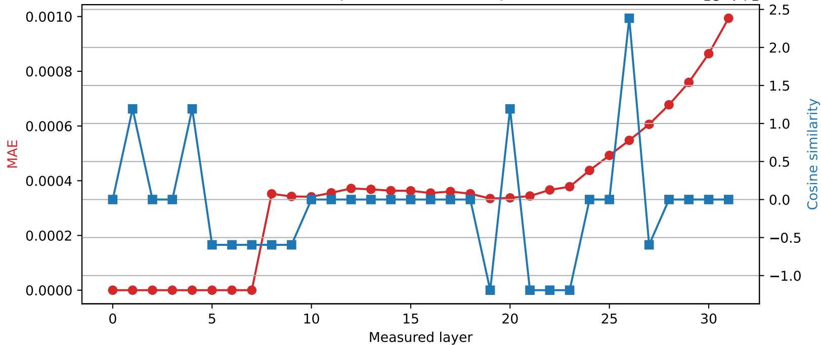
SmolLM2-360M | Quantized layer 7 | float32 \rightarrow int16
