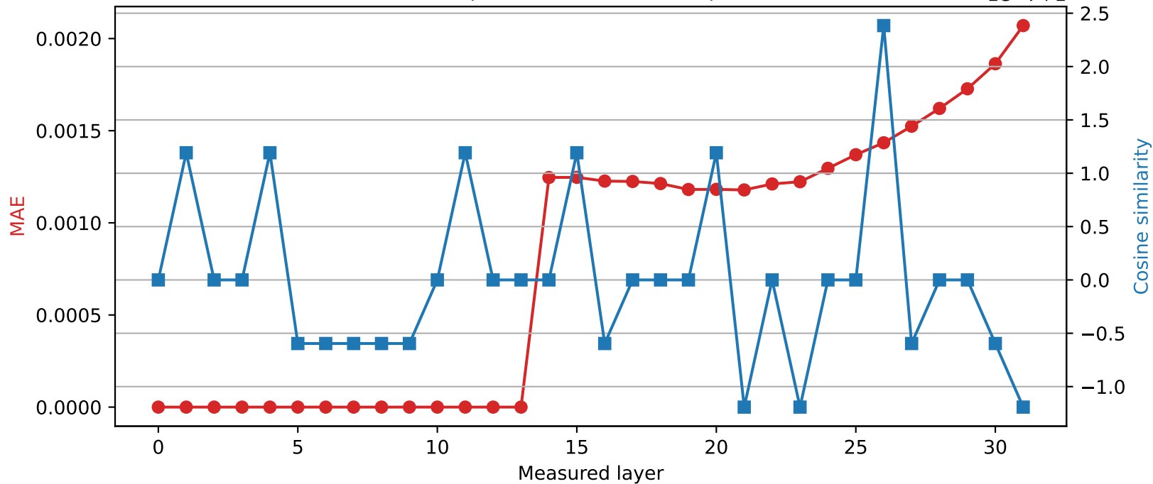
SmolLM2-360M | Quantized layer 13 | float32 \rightarrow int16
