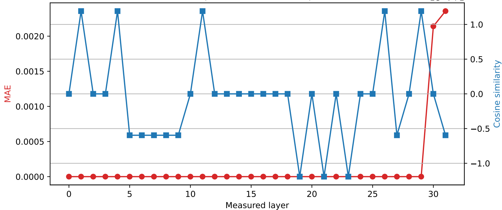
SmolLM2-360M | Quantized layer 29 | float32 \rightarrow int16
