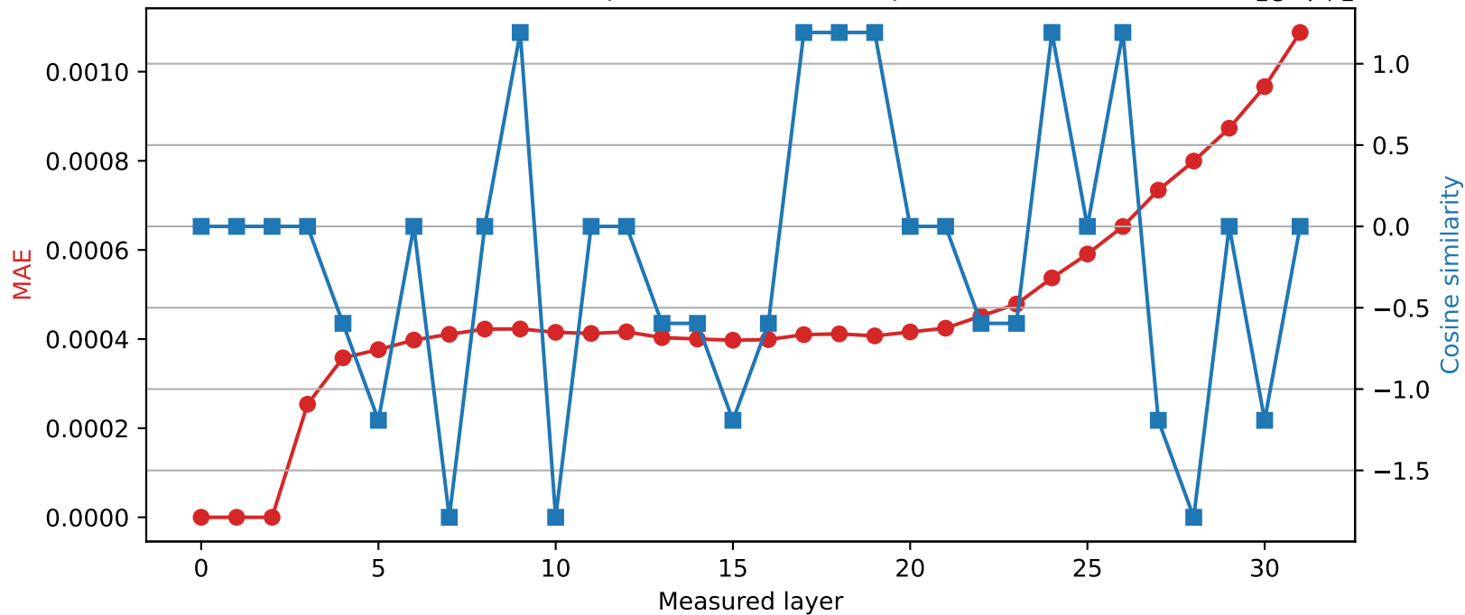
SmolLM2-360M | Quantized layer 2 | float32 → int16
