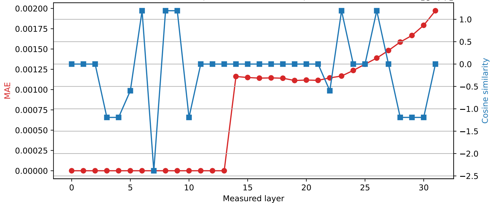
SmolLM2-360M | Quantized layer 13 | float32 \rightarrow int16
