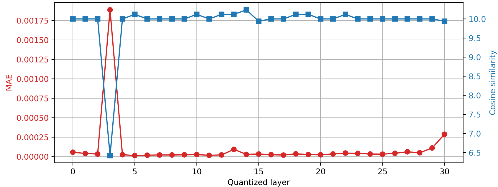
SmolLM2-360M | Prompt 4 Final RMSNorm output damage | float32 → int16
