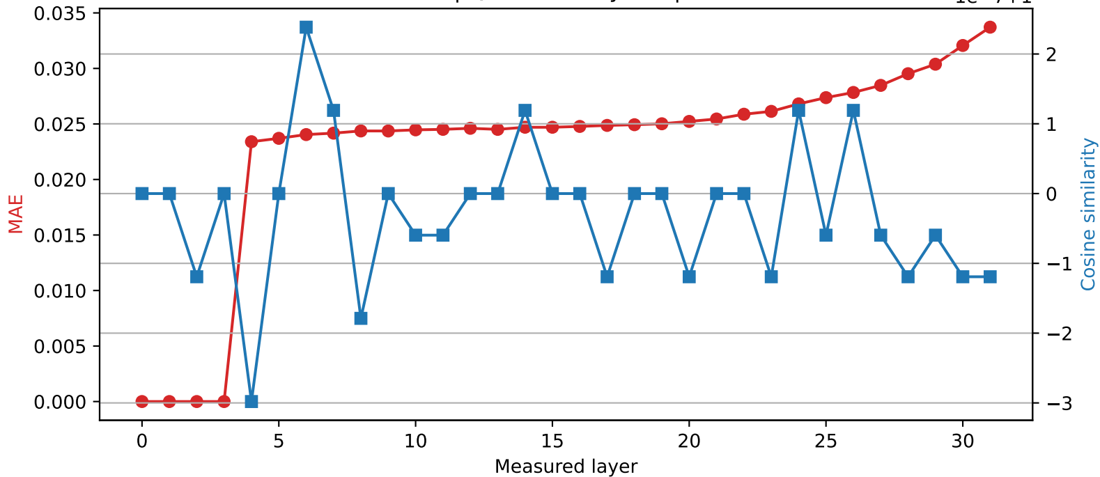
SmolLM2-360M | Quantized layer 3 | float32 → int16
