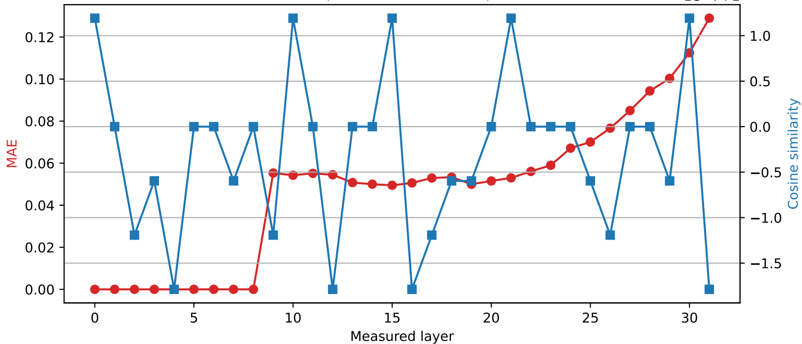
SmolLM2-360M | Quantized layer 8 | float32 → int8
