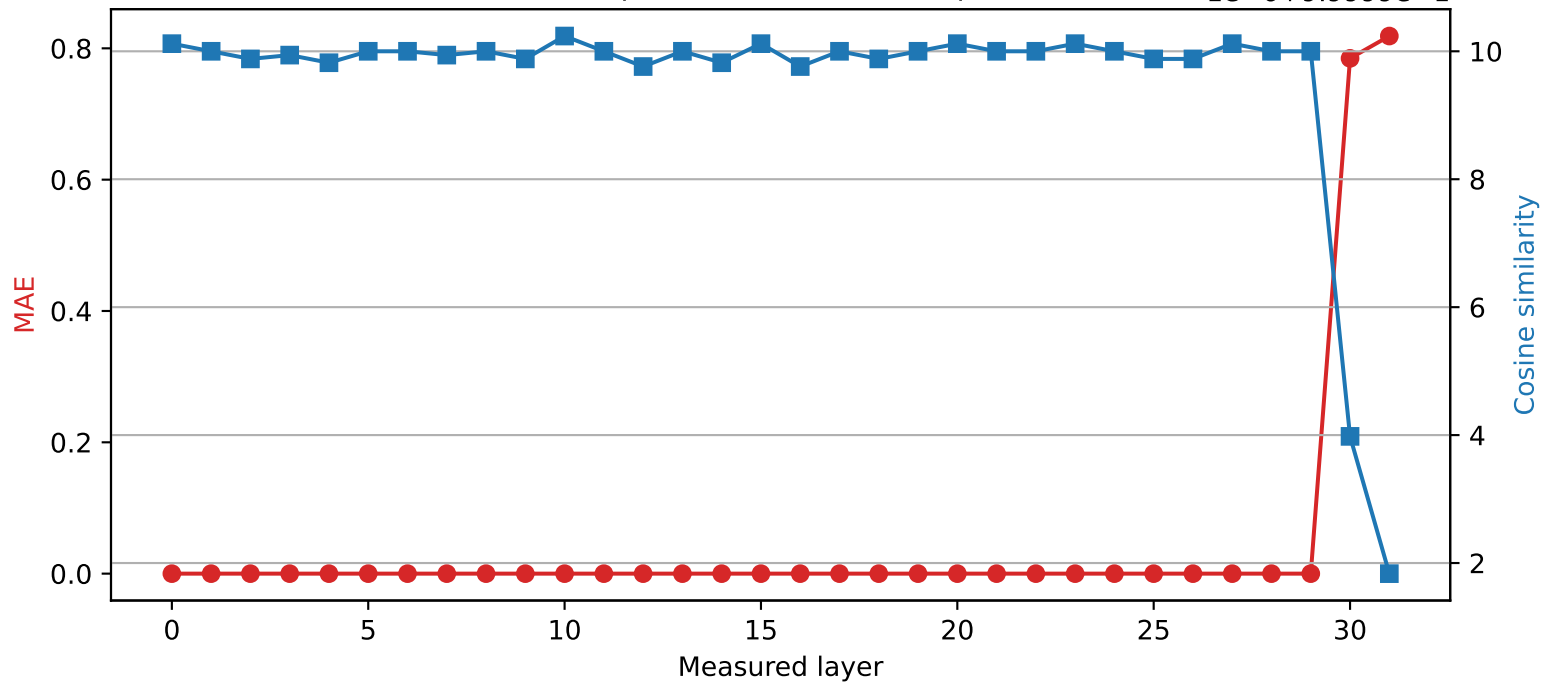
SmolLM2-360M | Quantized layer 29 | float32 \rightarrow int8 1e-6+9.9999e-1
