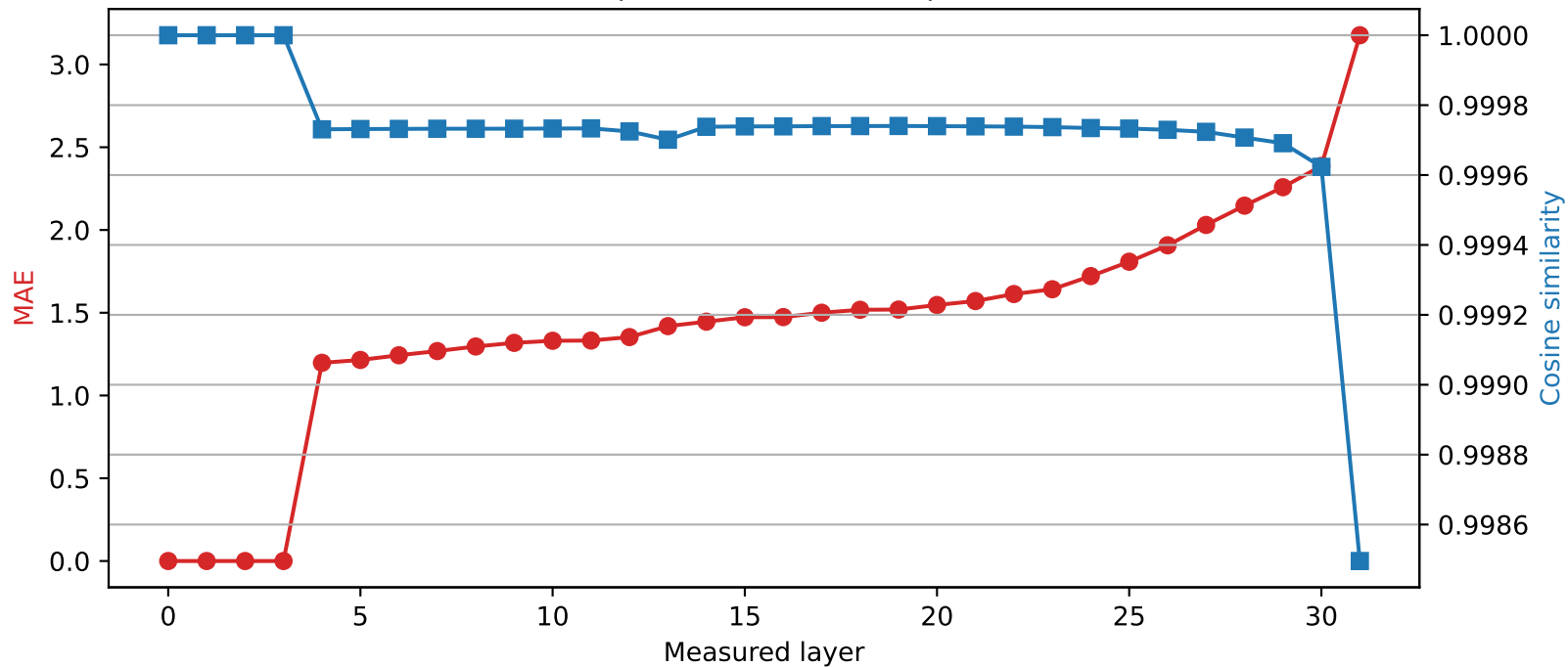
SmolLM2-360M | Quantized layer 3 | float32 → int8
