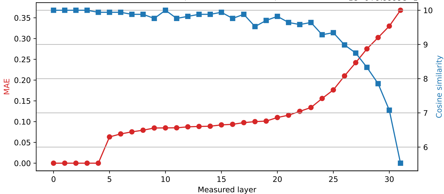
SmolLM2-360M | Quantized layer 4 | float32 → int8 1e-6+9.9999e-1
