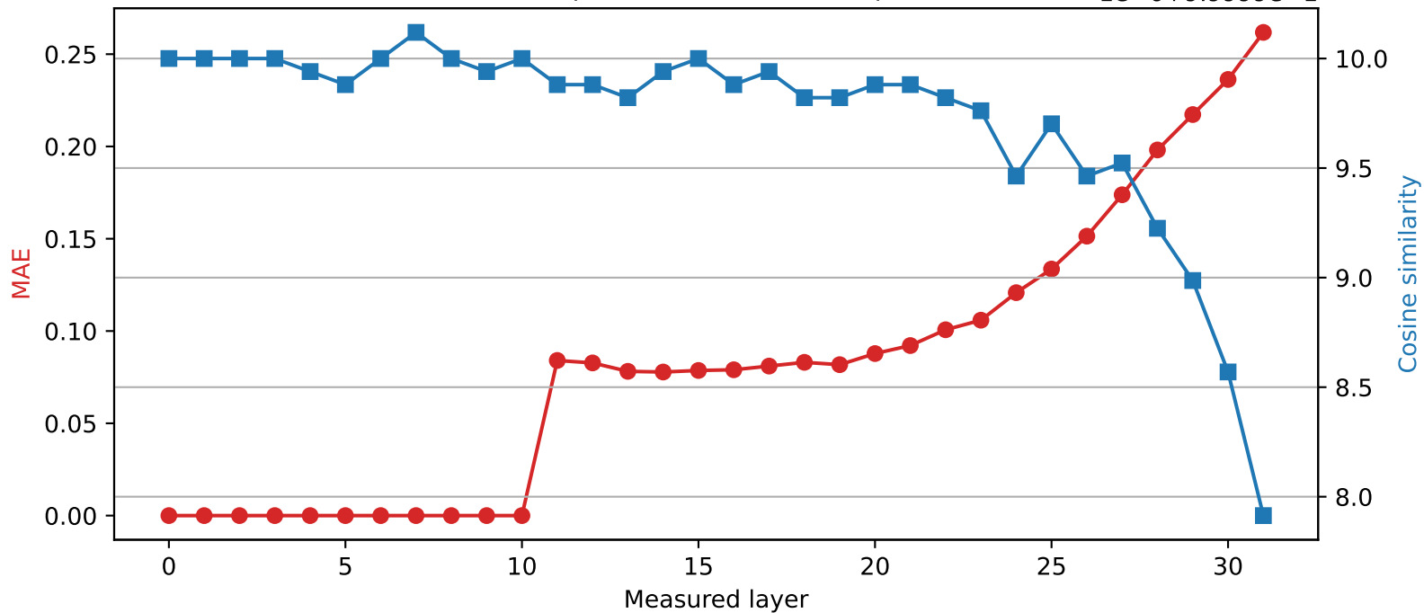
SmolLM2-360M | Quantized layer 10 | float32 \rightarrow int8 1e-6+9.9999e-1
