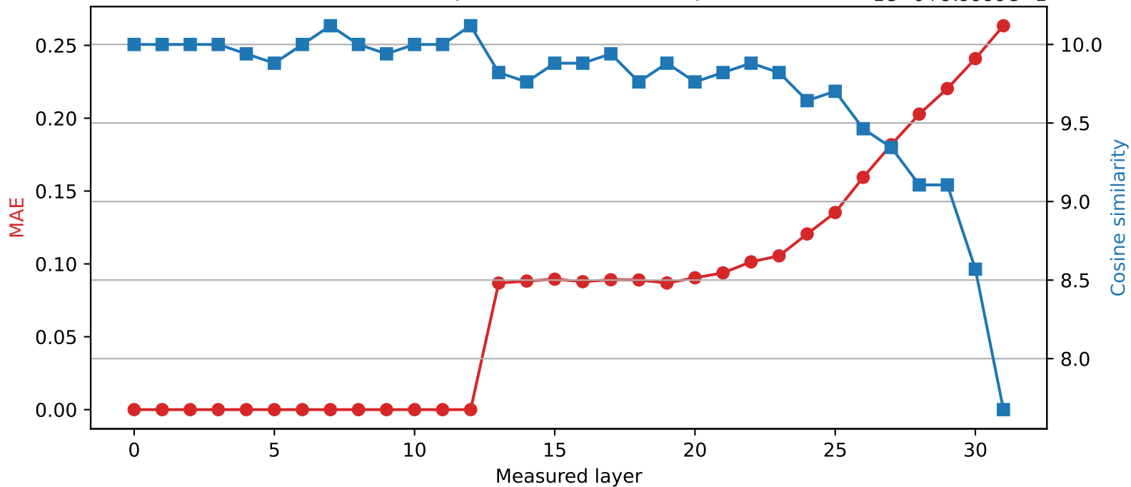
SmolLM2-360M | Quantized layer 12 | float32 \rightarrow int8 1e-6+9.9999e-1
