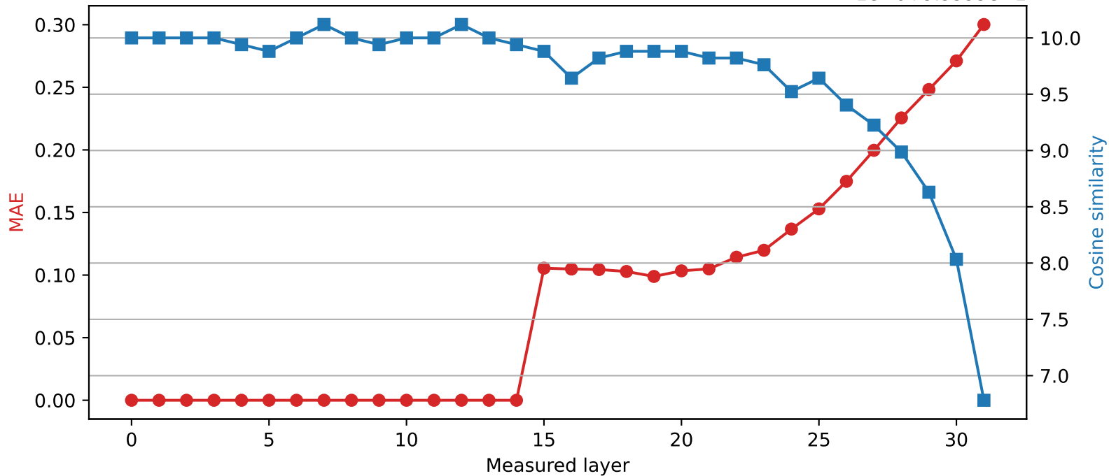
SmolLM2-360M | Quantized layer 14 | float32 \rightarrow int8 1e-6+9.9999e-1
