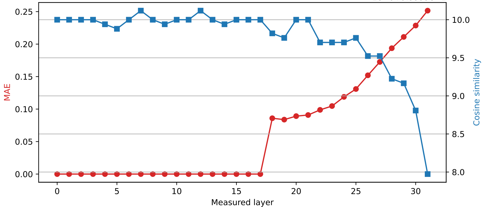
SmolLM2-360M | Quantized layer 17 | float32 \rightarrow int8 1e-6+9.9999e-1
