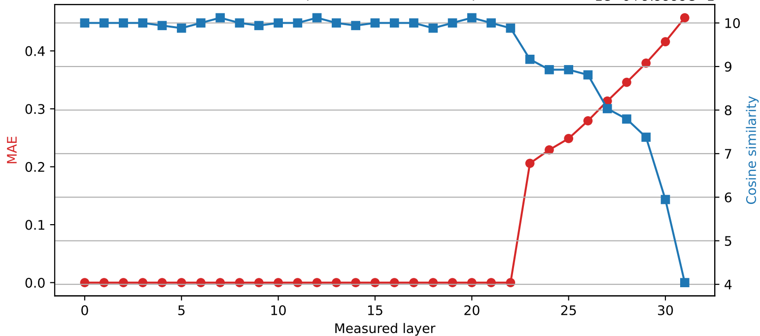
SmolLM2-360M | Quantized layer 22 | float32 \rightarrow int8 1e-6+9.9999e-1
