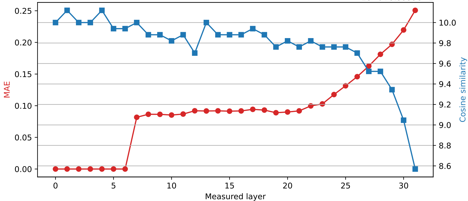
SmolLM2-360M | Quantized layer 6 | float32 \rightarrow int8 1e-6+9.9999e-1
