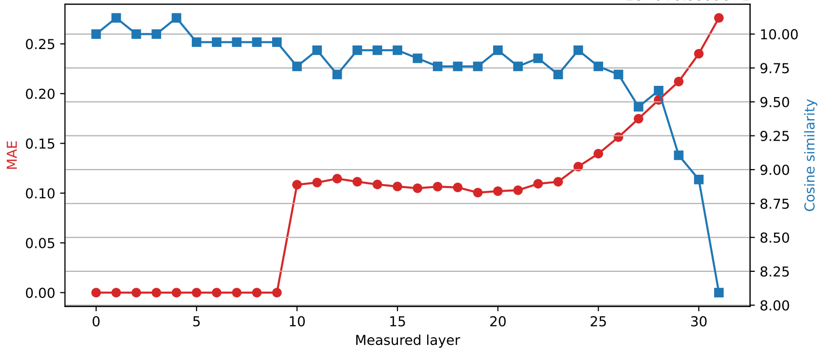
SmolLM2-360M | Quantized layer 9 | float32 \rightarrow int8 1e-6+9.9999e-1
