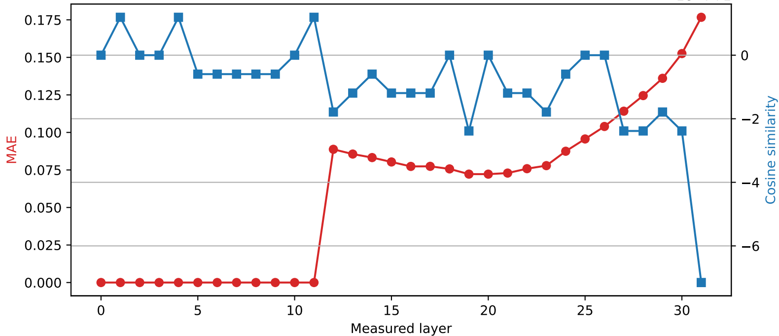
SmolLM2-360M | Quantized layer 11 | float32 → int8
