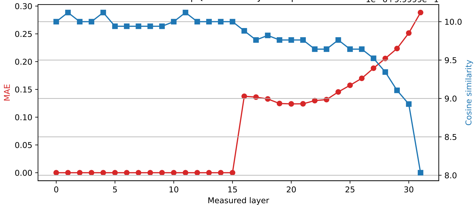
SmolLM2-360M | Quantized layer 15 | float32 \rightarrow int8 1e-6+9.9999e-1
