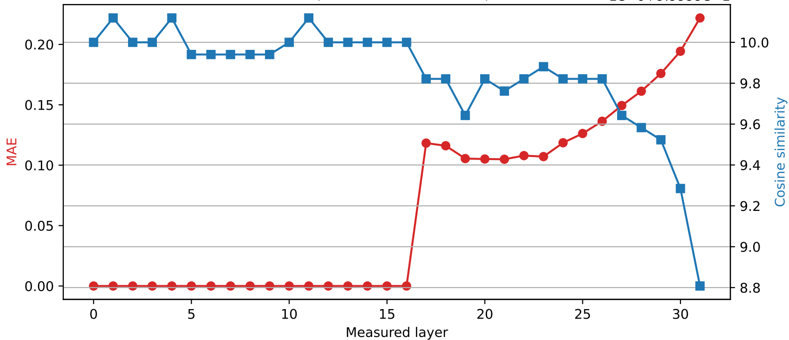
SmolLM2-360M | Quantized layer 16 | float32 \rightarrow int8 1e-6+9.9999e-1
