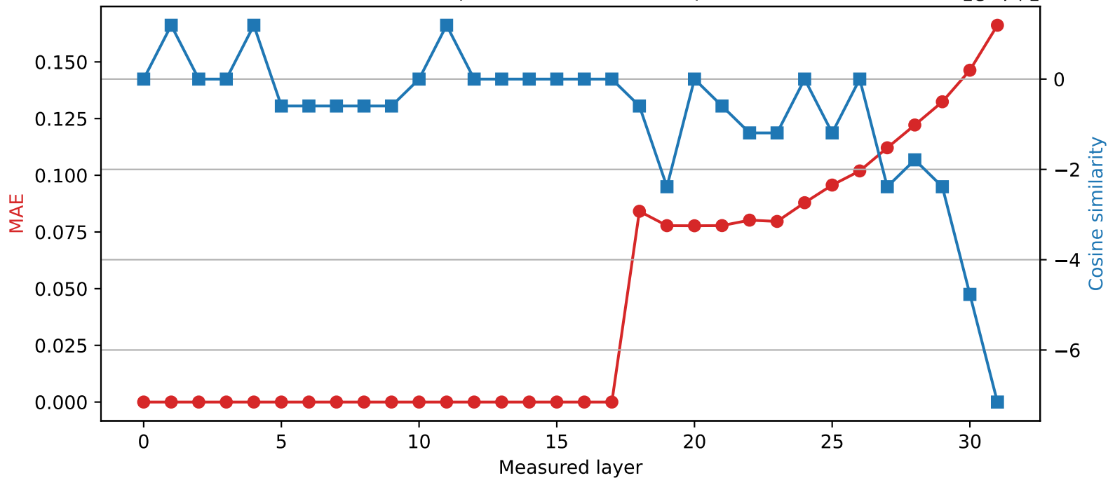
SmolLM2-360M | Quantized layer 17 | float32 → int8
