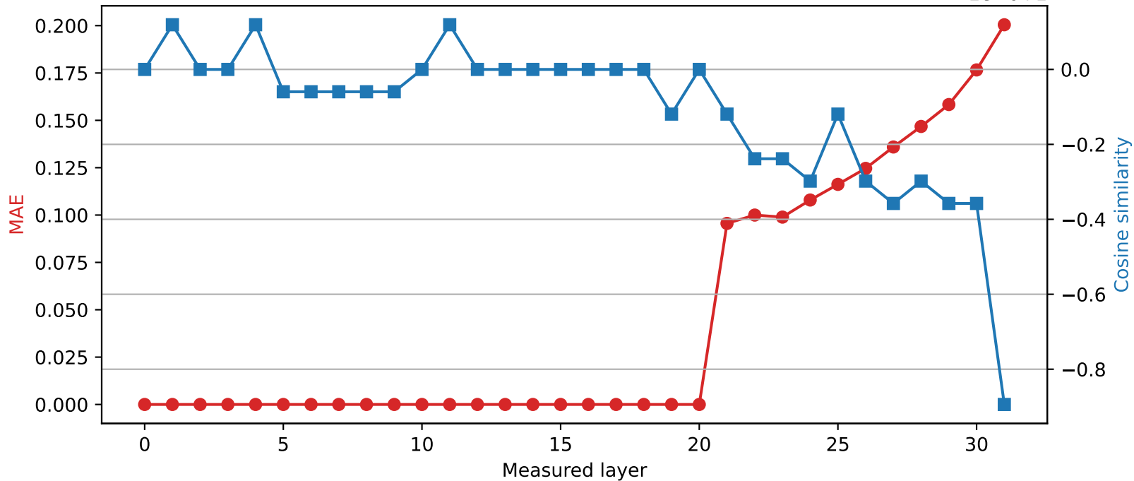
SmolLM2-360M | Quantized layer 20 | float32 \rightarrow int8
