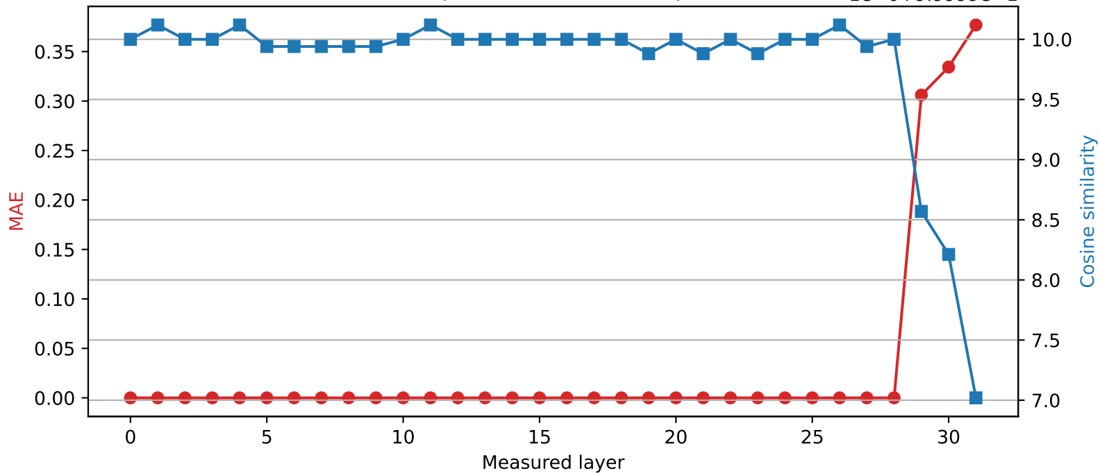
SmolLM2-360M | Quantized layer 28 | float32 → int8 1e-6+9.9999e-1
