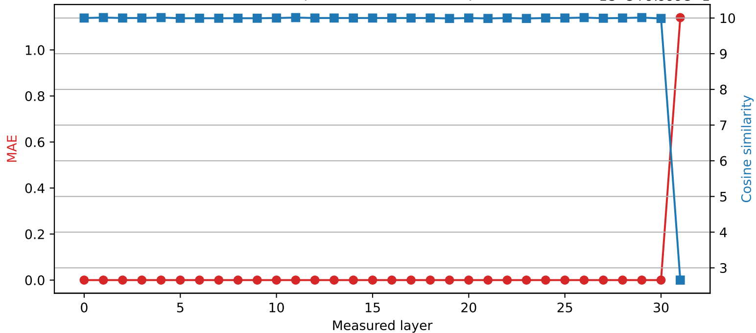
SmolLM2-360M | Quantized layer 30 | float32 → int8
