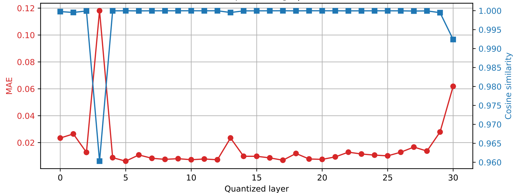
SmolLM2-360M | Prompt 3 Final RMSNorm output damage | float32 → int8
