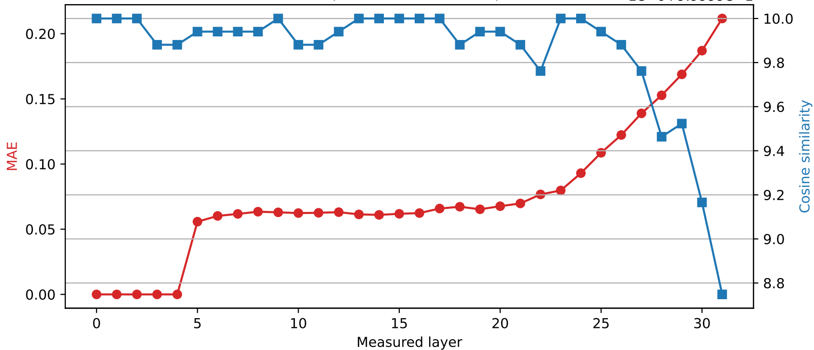
SmolLM2-360M | Quantized layer 4 | float32 \rightarrow int8 1e-6+9.9999e-1
