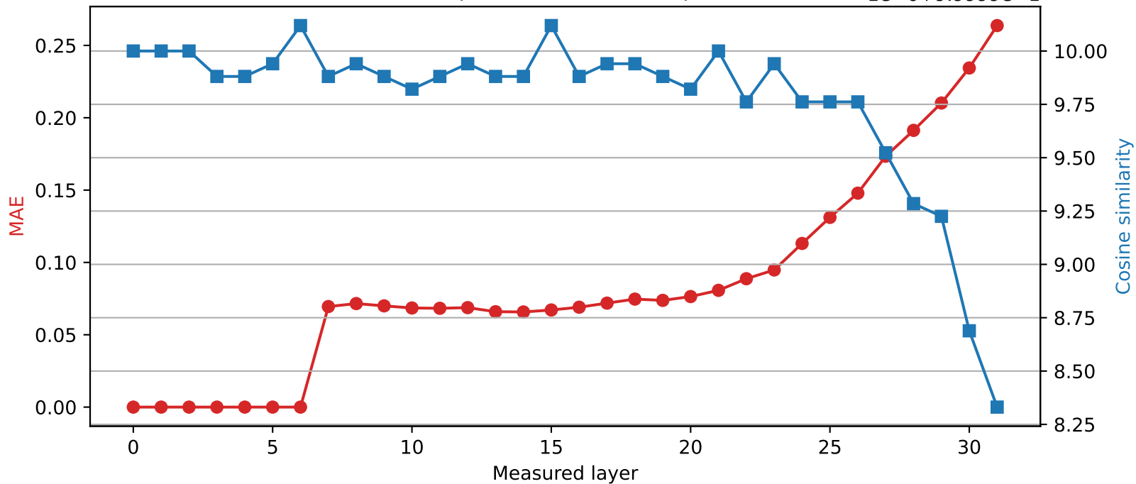
SmolLM2-360M | Quantized layer 6 | float32 → int8 1e-6+9.9999e-1
