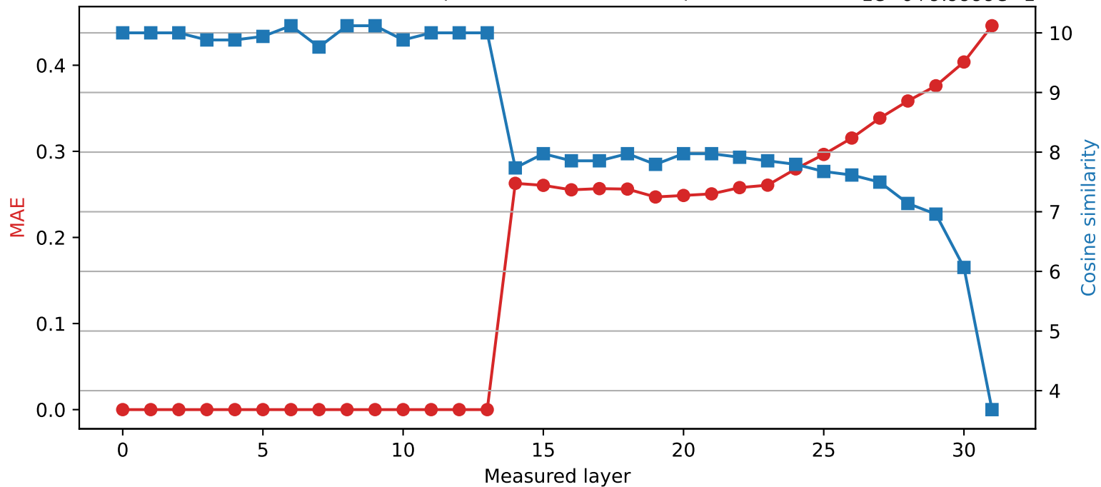
SmolLM2-360M | Quantized layer 13 | float32 \rightarrow int8 1e-6+9.9999e-1
