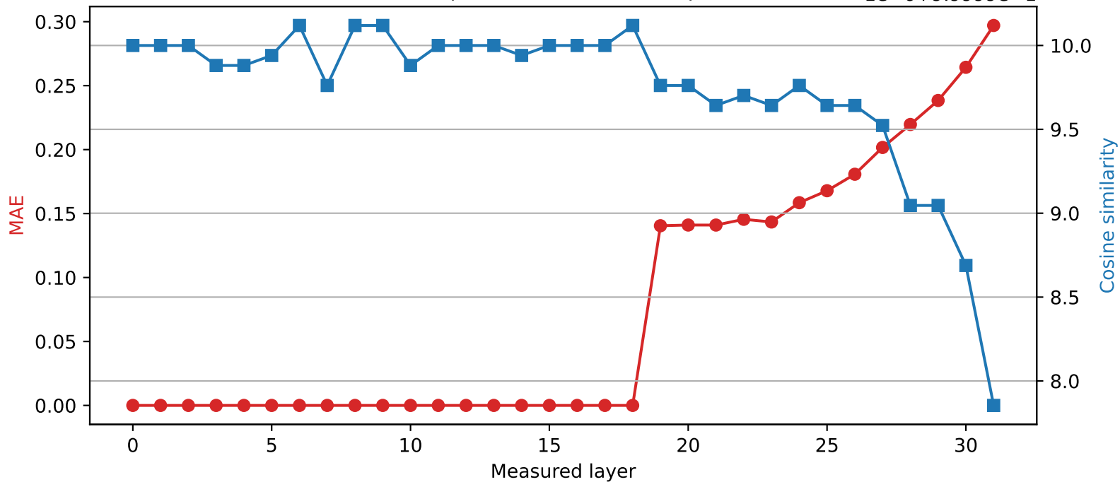
SmolLM2-360M | Quantized layer 18 | float32 \rightarrow int8 1e-6+9.9999e-1
