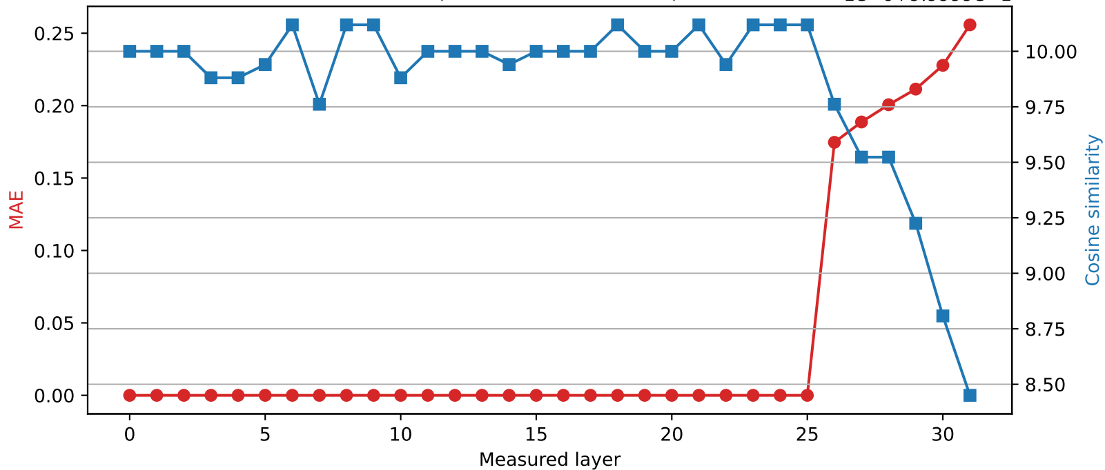
SmolLM2-360M | Quantized layer 25 | float32 \rightarrow int8 1e-6+9.9999e-1
