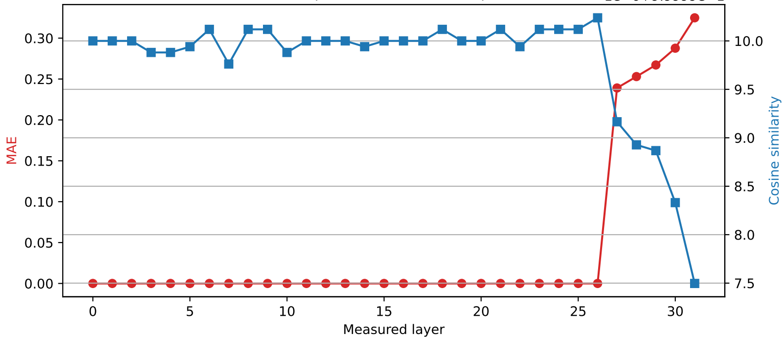
SmolLM2-360M | Quantized layer 26 | float32 → int8 1e-6 + 9.9999e-1
