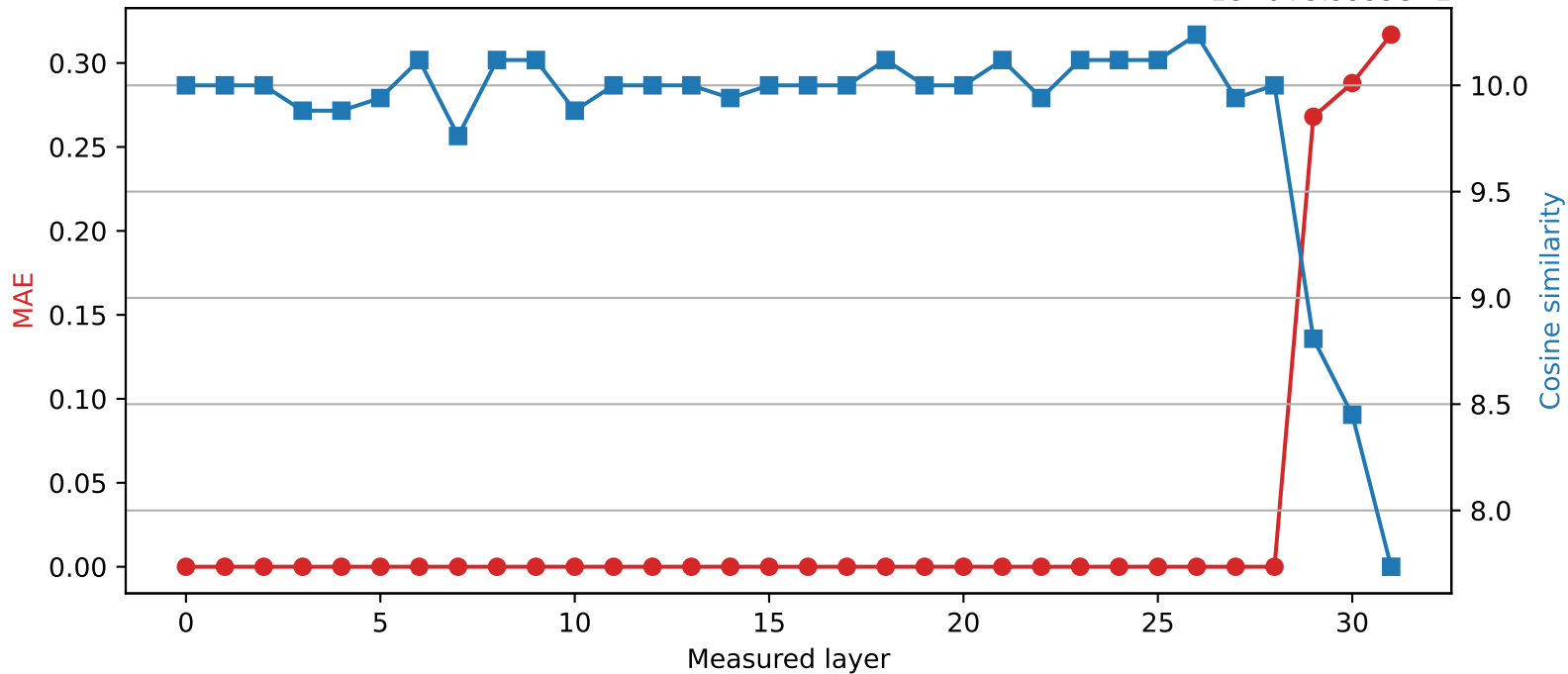
SmolLM2-360M | Quantized layer 28 | float32 \rightarrow int8 1e-6+9.9999e-1
