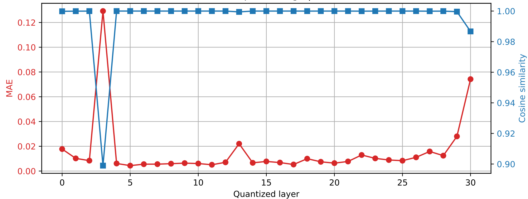
SmolLM2-360M | Prompt 4 Final RMSNorm output damage | float32 \rightarrow int8
