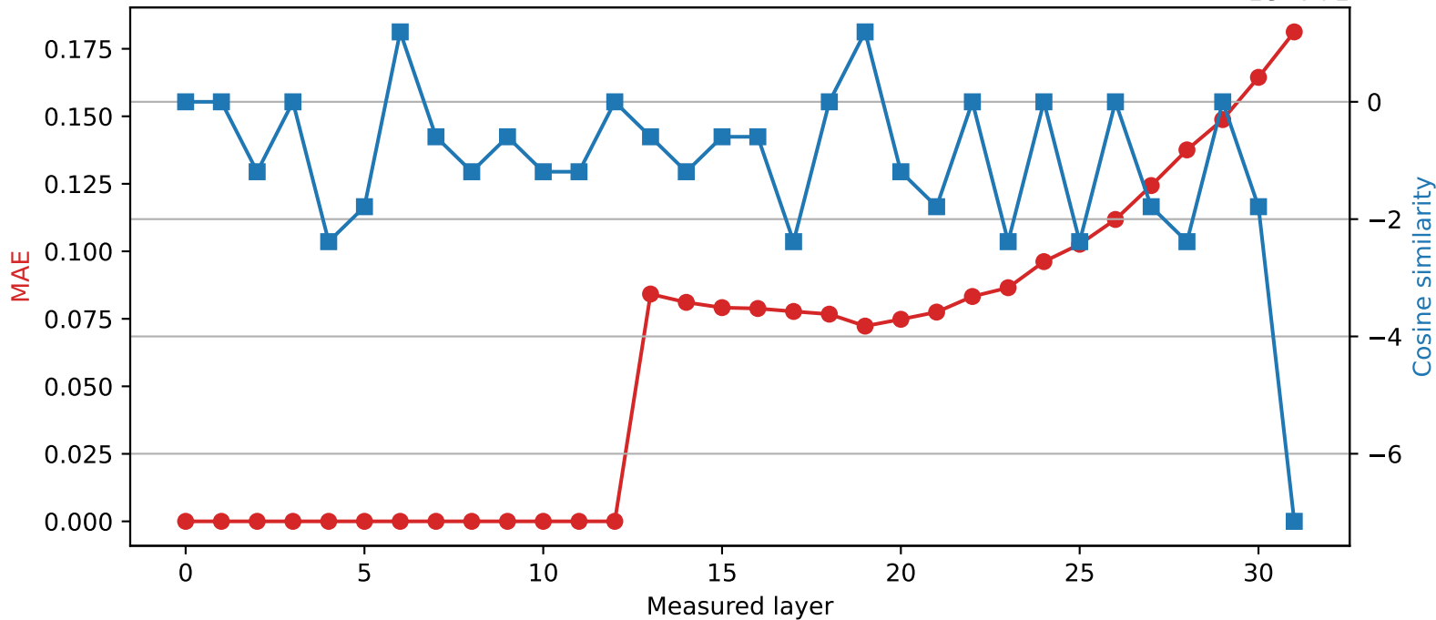
SmolLM2-360M | Quantized layer 12 | float32 → int8
