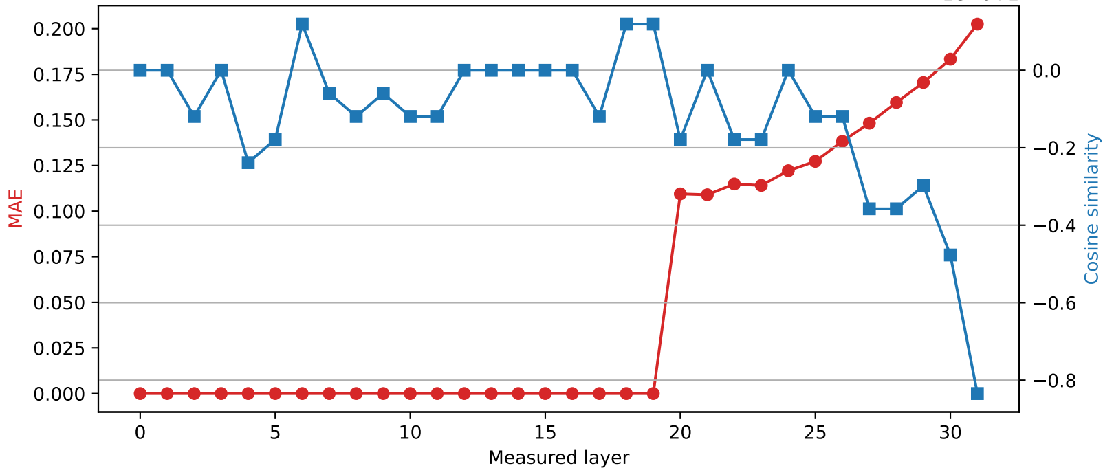
SmolLM2-360M | Quantized layer 19 | float32 → int8
